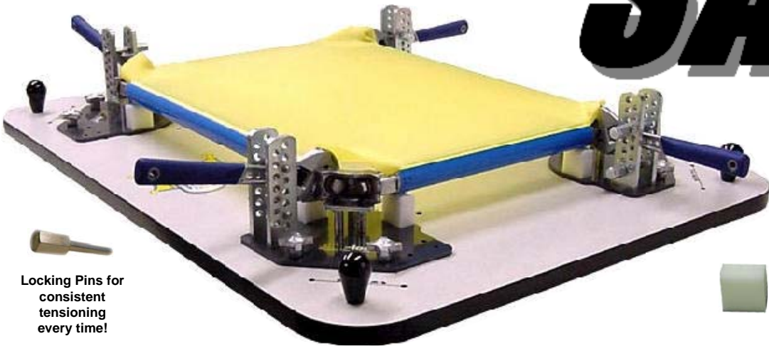
Low Friction Torsion Absorbing Pads prevent metal fatigue in your frames.
